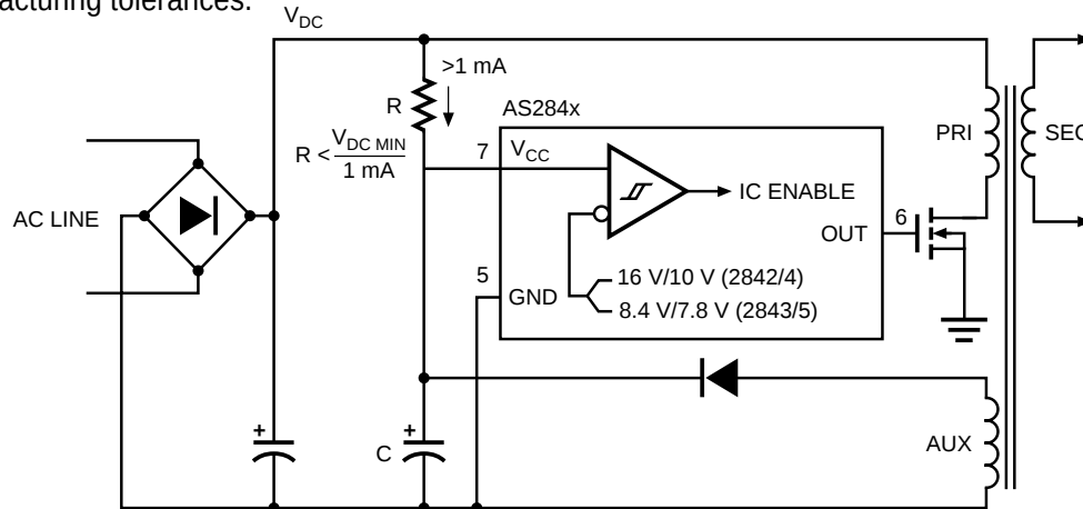
Figure 14. Bootstrap Circuit
