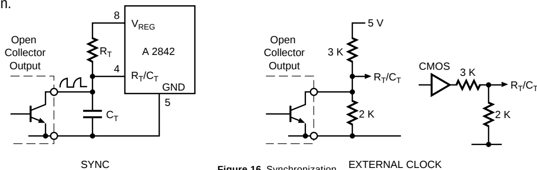
Figure 16. Synchronization EXTERNAL CLOCK
