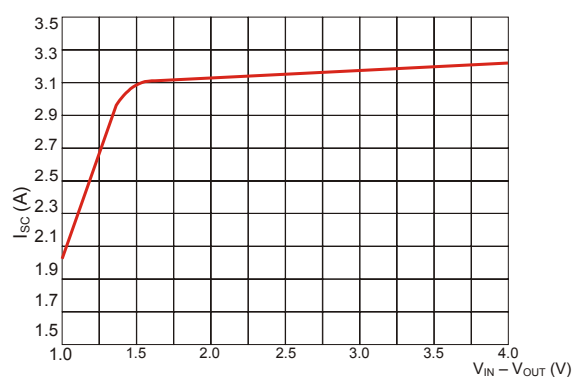
Figure 6. Short Circuit Current vs. V_{IN} - V_{OUT}
