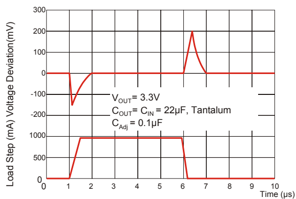
Figure 5. Transient Response
