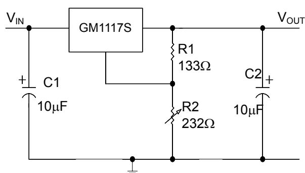
Adjustable Regulator
