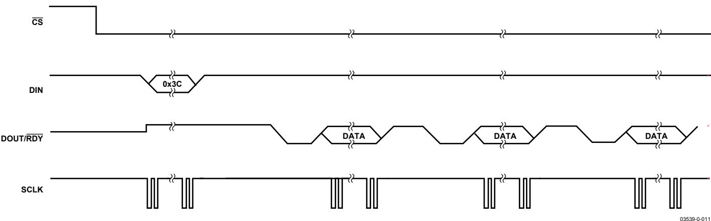
Figure 13. Continuous Read
