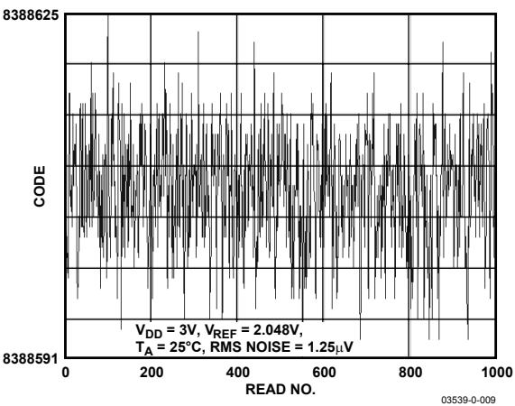
Figure 8. AD7789 Noise Plot
