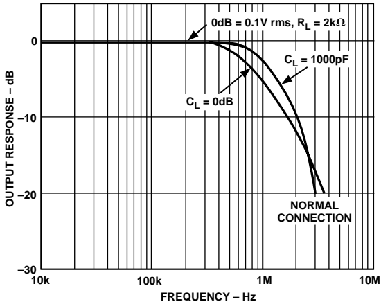
Figure 15. Frequency Response
