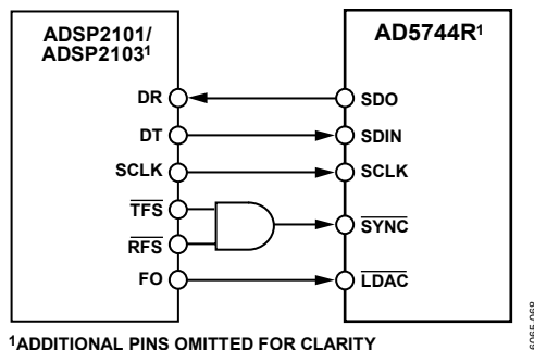
Figure 43. AD5744R to ADSP2101/ADSP2103 Interface
