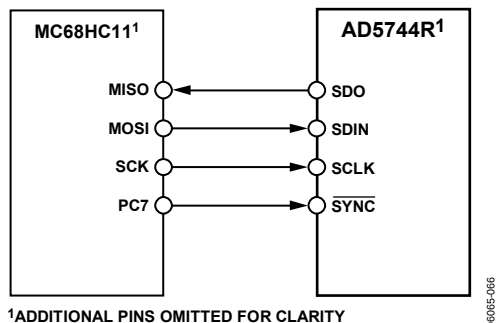
Figure 41. AD5744R to MC68HC11 Interface
