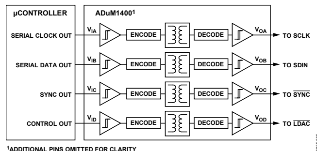
Figure 40. Isolated Interface
