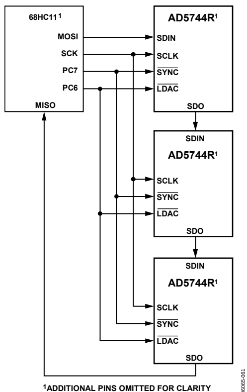
Figure 36. Daisy Chaining the AD5744R
