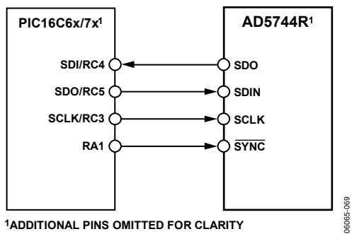
Figure 44. AD5744R to PIC16C6x/7x Interface
