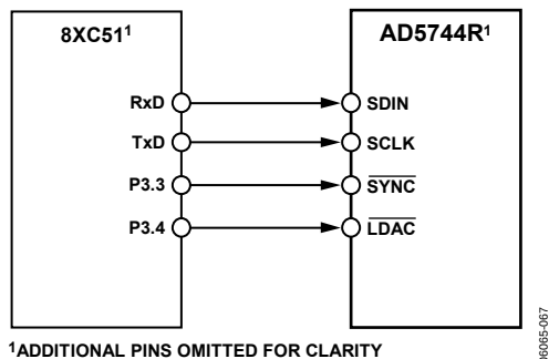
Figure 42. AD5744R to 8XC51 Interface
