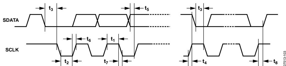
Figure 2. I²C Timing
