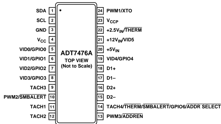
Figure 3. Pin Configuration
