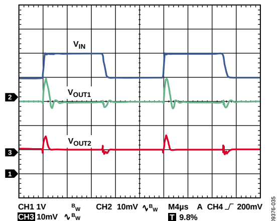
Figure 55. Transient Line Response, V_{OUTx} = 1.2\text{V} and 1.8\text{V} , V_{IN} = 4\text{V} to 5\text{V} , I_{LOAD} = 10\text{mA}
