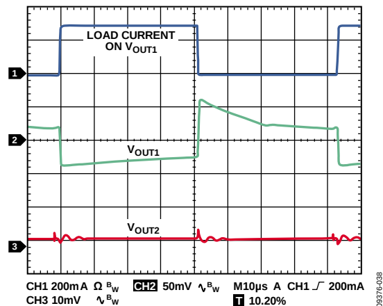
Figure 58. Transient Load Response, V_{OUTx} = 3.3\text{V} , I_{LOAD} = 1\text{mA} to 300\text{mA} ; V_{OUTx} = 2.8\text{V} , I_{LOAD} = 1\text{mA}
