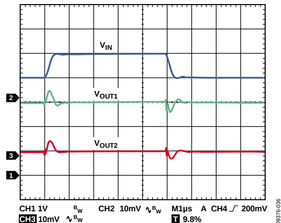
Figure 56. Transient Line Response, V_{OUTx} = 3.3\text{V} and 2.8\text{V} , V_{IN} = 4\text{V} to 5\text{V} , I_{LOAD} = 300\text{mA}
