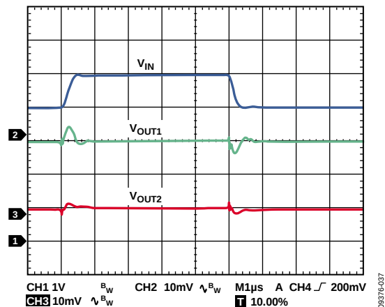
Figure 57. Transient Line Response, V_{OUTx} = 1.2\text{V} and 1.8\text{V} , V_{IN} = 4\text{V} to 5\text{V} , I_{LOAD} = 300\text{mA}
