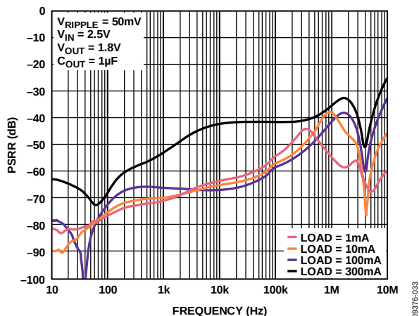
Figure 53. Power Supply Rejection Ratio vs. Frequency, V_{IN} = 2.5\text{V} , V_{OUTx} = 1.8\text{V}
