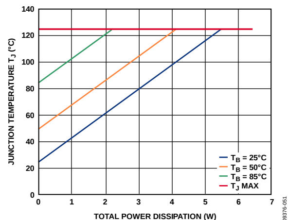
Figure 75. 8-Lead LFCSP, T_A = 85^\circ\text{C}
