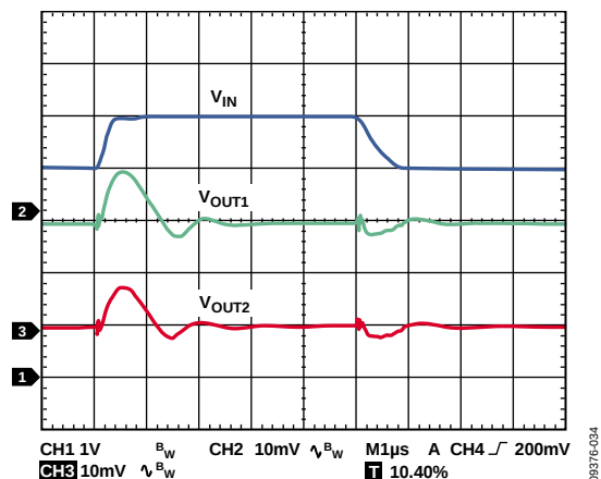
Figure 54. Transient Line Response, V_{OUTx} = 3.3\text{V} and 2.8\text{V} , V_{IN} = 4\text{V} to 5\text{V} , I_{LOAD} = 10\text{mA}
