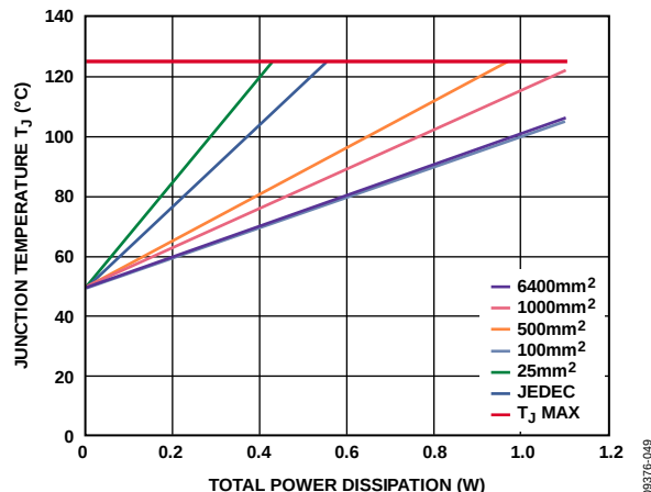
Figure 73. 8-Lead LFCSP, T_A = 50^\circ\text{C}
