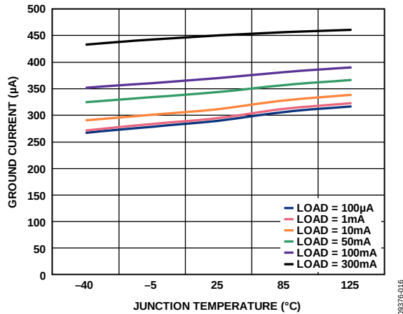
Figure 36. Ground Current vs. Junction Temperature, Dual Output, Includes 200 \mu A for Output Dividers, ADP223/ADP225
