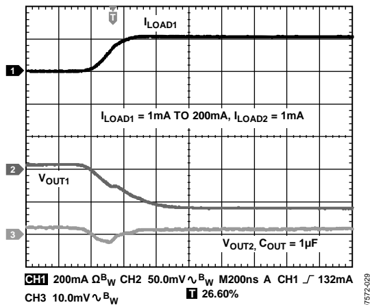
Figure 29. Output Transient Response I_{\text{LOAD1}} = 1 \text{ mA to } 200 \text{ mA} , I_{\text{LOAD2}} = 1 \text{ mA} CH1 = I_{\text{LOAD1}} , CH2 = V_{\text{OUT1}} , CH3 = V_{\text{OUT2}} , C_{\text{OUT}} = 1 \mu\text{F}
