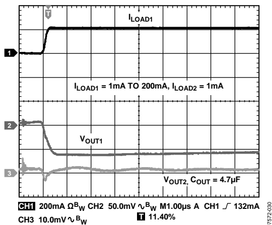
Figure 30. Output Transient Response I_{\text{LOAD1}} = 1 \text{ mA to } 200 \text{ mA} , I_{\text{LOAD2}} = 1 \text{ mA} CH1 = I_{\text{LOAD1}} , CH2 = V_{\text{OUT1}} , CH3 = V_{\text{OUT2}} , C_{\text{OUT}} = 4.7 \mu\text{F}
