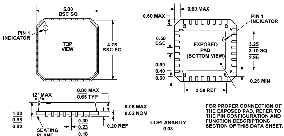
Figure 36. 32-Lead Lead Frame Chip Scale Package [LFCSP_VQ] 5 mm x 5 mm Body, Very Thin Quad (CP-32-2) Dimensions shown in millimeters
