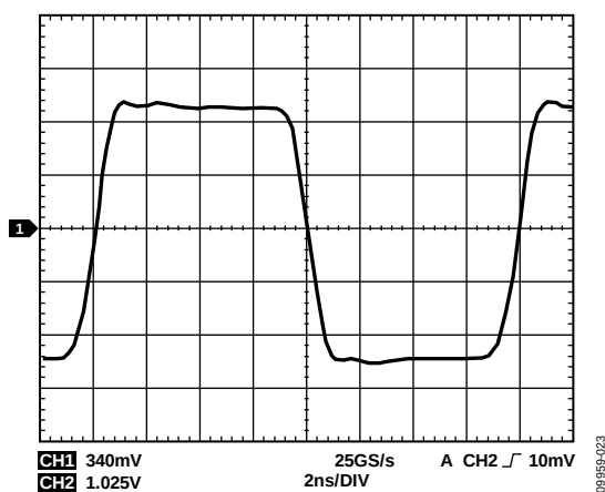
Figure 23. Large Signal Pulse Response, A_V = 15.5 dB
