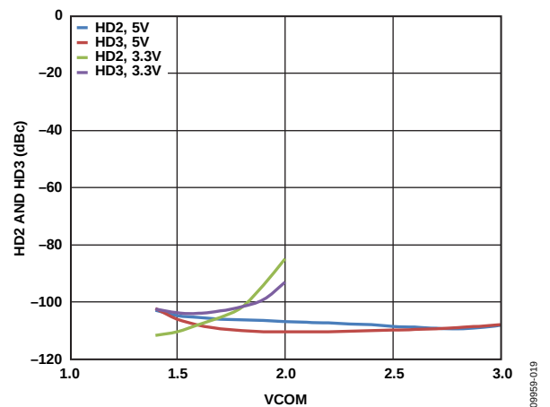
Figure 20. Harmonic Distortion (HD2/HD3) vs. V_{COM} , A_V = 6 dB, V_{POS} = 3.3 V and V_{POS} = 5 V
