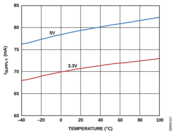
Figure 29. I_{SUPPLY} vs. Temperature, R_L = 200 \Omega , A_V = 6 dB, V_{POS} = 3.3 V and V_{POS} = 5 V
