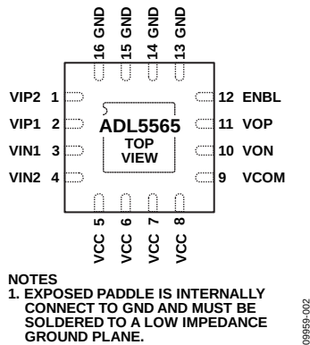
Figure 2. Pin Configuration
