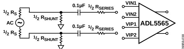
Figure 36. Gain Adjustment Using a Series Resistor
