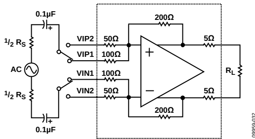
Figure 30. Basic Structure
