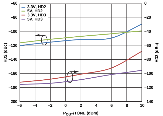
Figure 19. Harmonic Distortion vs. Output Power per Tone, Frequency = 100 MHz, R_L = 200 \Omega , V_{POS} = 3.3 V and V_{POS} = 5 V
