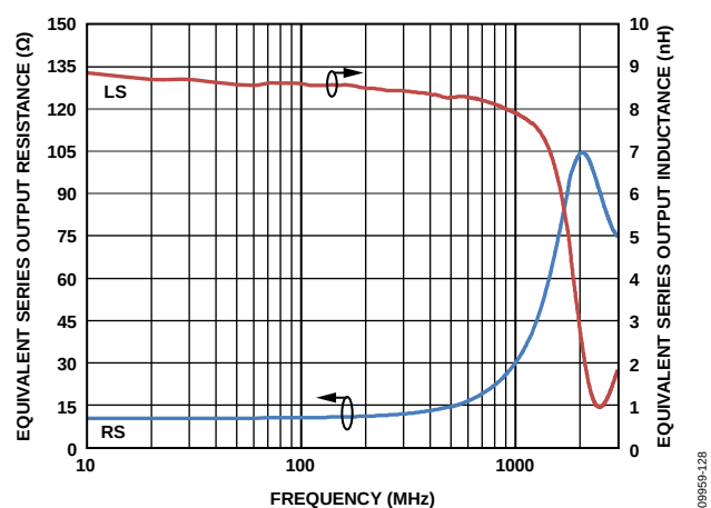
Figure 28. S22 Equivalent RLC Parallel Network, A_V = 6 dB
