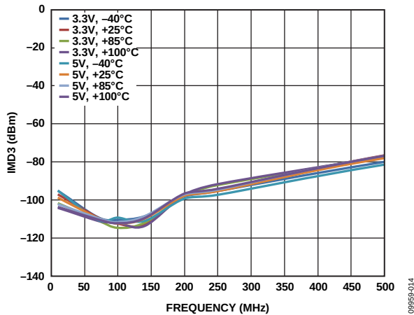
Figure 15. IMD3 vs. Frequency, Over Temperature, Output Level at 2 V p-p Composite, R_L = 200 \Omega , A_V = 6 dB, V_{POS} = 3.3 V and V_{POS} = 5 V, Four Temperatures
