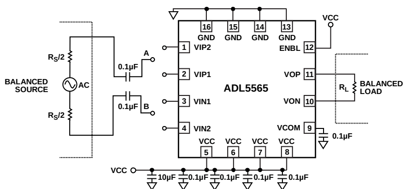
Figure 31. Basic Connections
