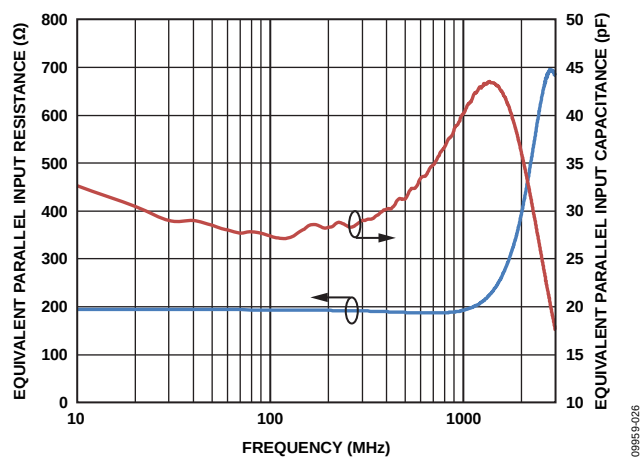
Figure 27. S11 Equivalent RLC Parallel Network, A_V = 6 dB
