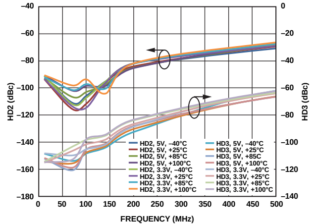
Figure 18. Harmonic Distortion (HD2/HD3) vs. Frequency, Over Temperature, Output Level at 2 V p-p Composite, R_L = 200 \Omega , A_V = 6 dB, V_{POS} = 3.3 V and V_{POS} = 5 V, Four Temperatures
