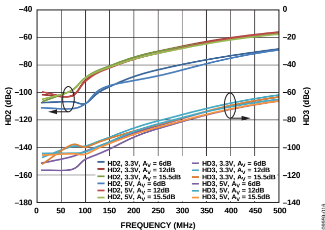
Figure 17. Harmonic Distortion (HD2/HD3) vs. Frequency, Output Level at 2 V p-p Composite, R_L = 200 \Omega , V_{POS} = 3.3 V and V_{POS} = 5 V
