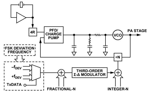
Figure 27. FSK Implementation
