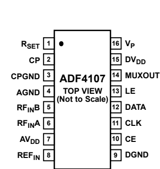
Figure 3. Pin Configuration, TSSOP
