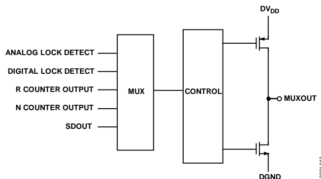
Figure 12. MUXOUT Circuit
