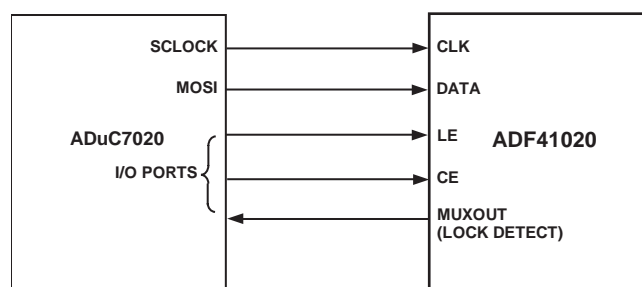
Figure 18. ADuC7020-to-ADF41020 Interface
