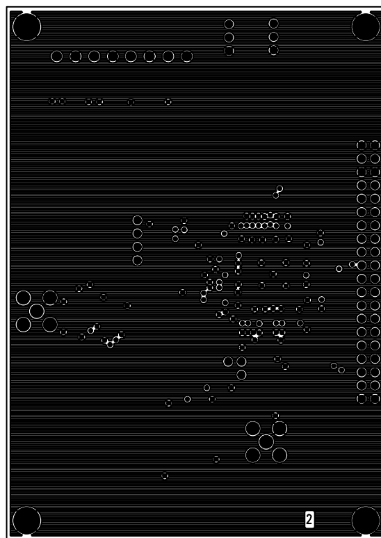
Figure 50. PCB Ground Layer
