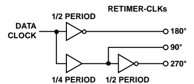
Figure 95. RETIMER-CLK Phases
