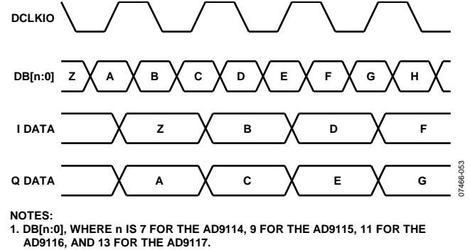
Figure 91. Timing Diagram with IFIRST = 1, IRISING = 0
