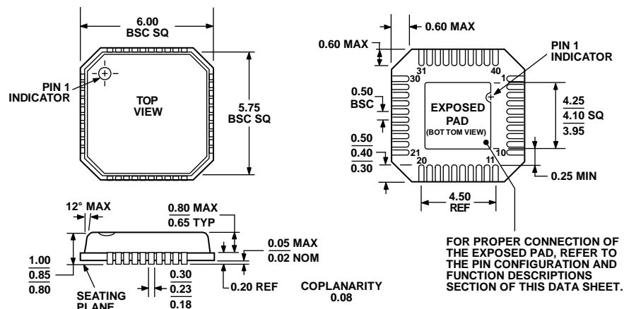
Figure 111. 40-Lead Lead Frame Chip Scale Package [LFCSP_VQ]
