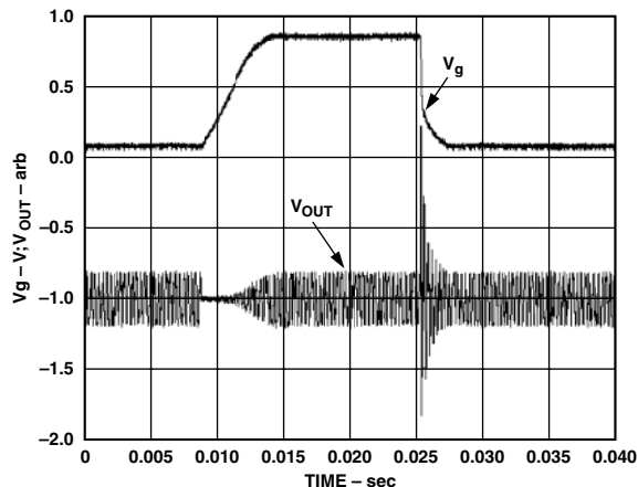
Figure 15. AGC Dynamic Response: 8367 AGC with an External Detector
