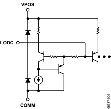
Figure 6. LO Decoupling Pin
