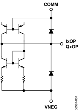
Figure 8. Output Drivers
