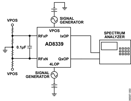
Figure 51. PSRR
