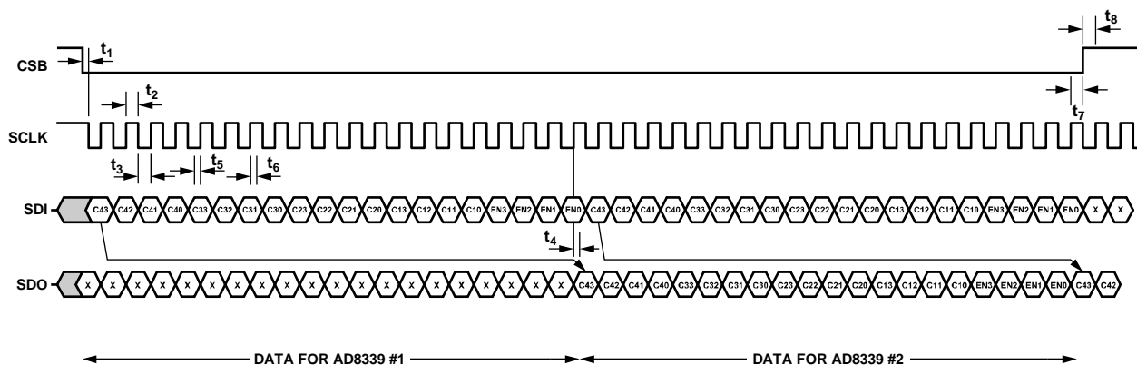
Figure 57. Timing Diagram
