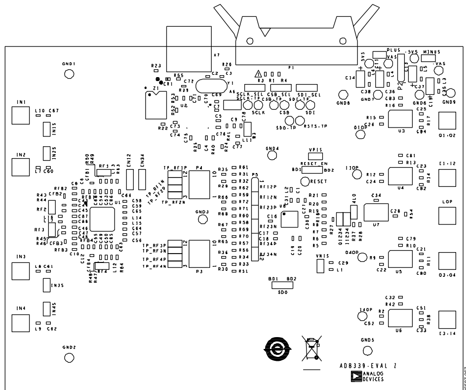
Figure 69. AD8339-EVALZ Assembly
