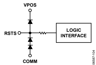
Figure 4. RSTS Logic Input
