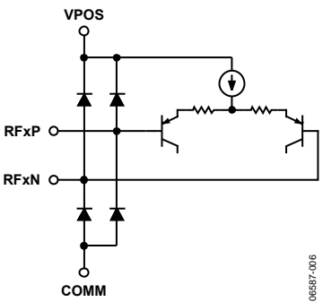
Figure 7. RF Inputs
