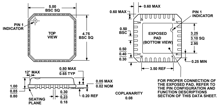
Figure 71. 32-Lead Lead Frame Chip Scale Package [LFCSP_VQ] 5 mm × 5 mm Body, Very Thin Quad (CP-32-2) Dimensions shown in millimeters
