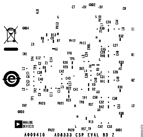
Figure 68. Component Side Silkscreen
