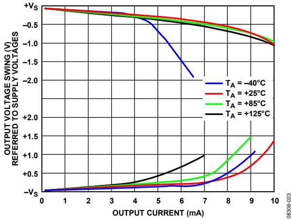
Figure 23. Output Voltage Swing vs. I_{OUT} and Temperature, V_S = \pm 15V
