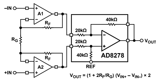
Figure 56. Low Power Precision Instrumentation Amplifier
