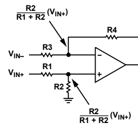
Figure 46. Voltage Division in the Difference Amplifier Configuration
