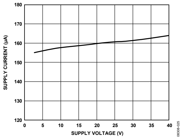
Figure 25. Supply Current vs. Single-Supply Voltage, V_{IN} = 0V , V_{REF} = 0V
