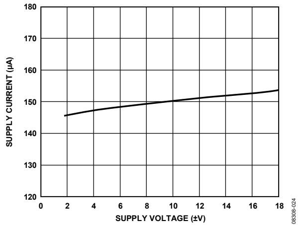
Figure 24. Supply Current vs. Dual-Supply Voltage, V_{IN} = 0V
