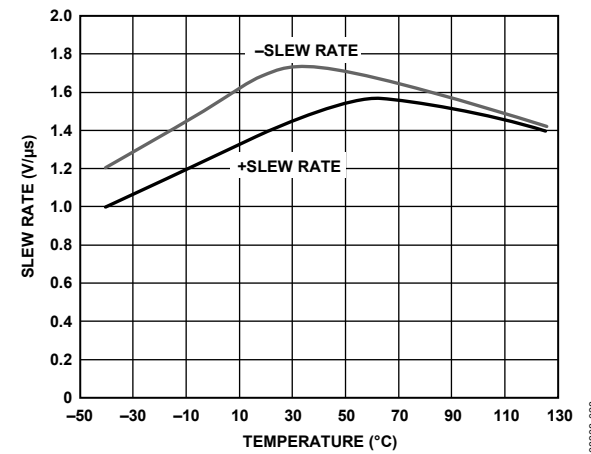
Figure 28. Slew Rate vs. Temperature, V_{IN} = 20V p-p, 1 kHz
