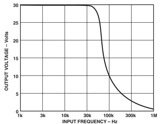
TPC 21. Large Signal Frequency Response
