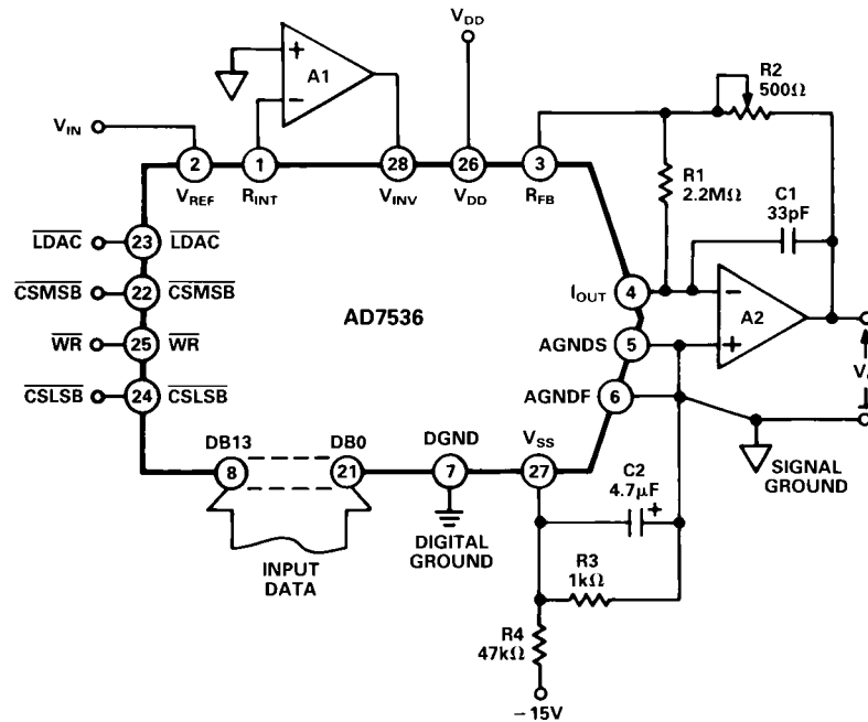
Figure 5. AD7536 Operation
