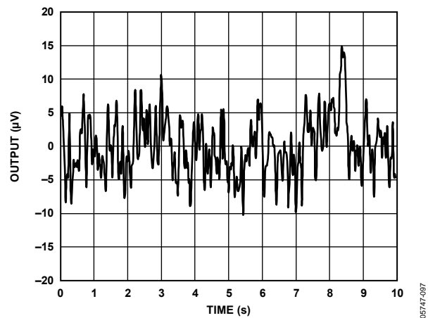
Figure 21. 0.1 Hz to 10 Hz DAC Output Noise (Code 800)
