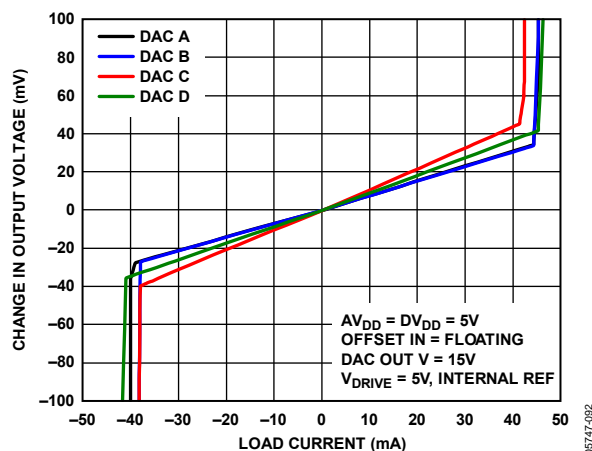
Figure 26. DAC Output Voltage vs. Load Current, Input Code = x800
