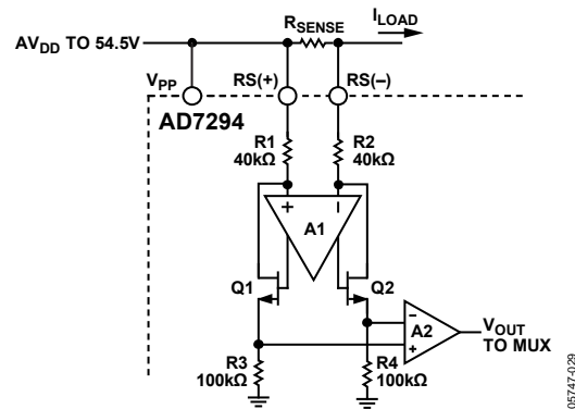
Figure 41. High-Side Current Sense
