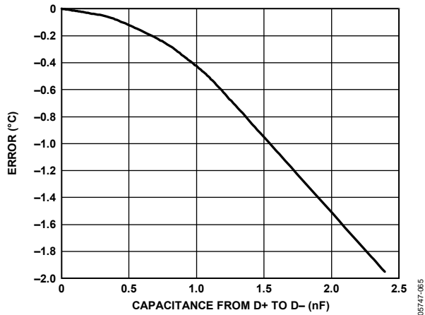
Figure 29. Temperature Error vs. Capacitor Between D+ and D-
