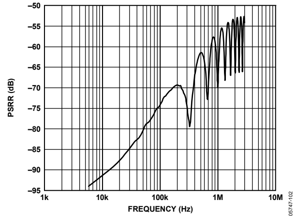
Figure 32. I_{\text{SENSE}} Power Supply Rejection Ratio vs. Supply Ripple Frequency Without V_{\text{PP}} Supply Decoupling Capacitors for a 500 mV Ripple
