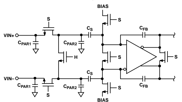
Figure 26. Switched-Capacitor Input
