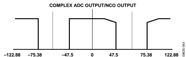
Figure 39. Example AD6649 95 MHz Bandwidth Input Signal Tuned to DC Using the NCO (NCO Frequency = 61.44 MHz)
