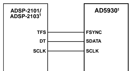
Figure 36. ADSP-2101/ADSP-2103 to AD5930 Interface
