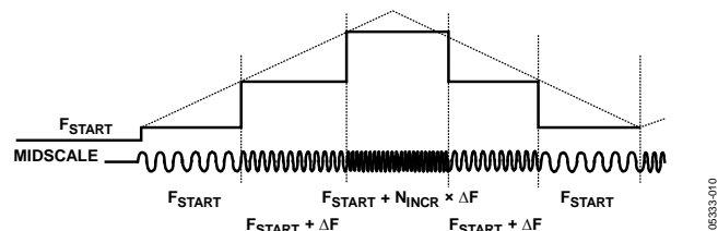
Figure 32. Triangular-Sweep Profile
