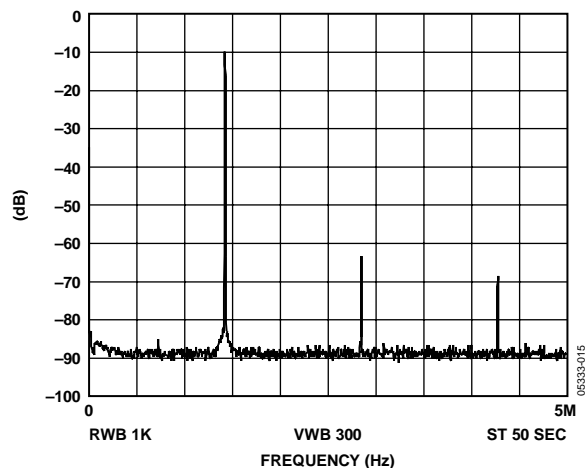
Figure 23. f_{MCLK} = 10 \text{ MHz} ; f_{OUT} = 1.43 \text{ MHz} = f_{MCLK}/7 , Frequency Word = 249249
