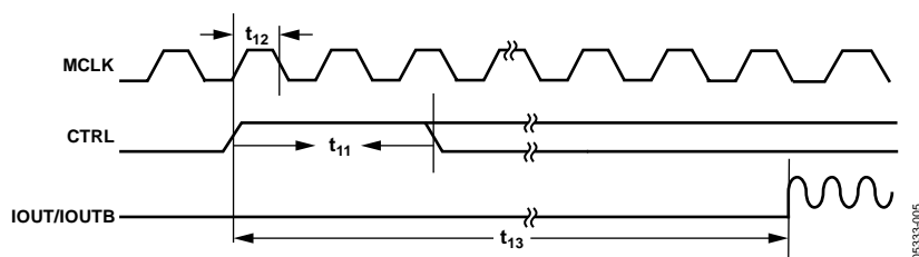
Figure 5. CTRL Timing
