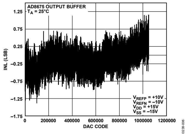
Figure 6. Integral Nonlinearity Error vs. DAC Code, \pm 10 V Span
