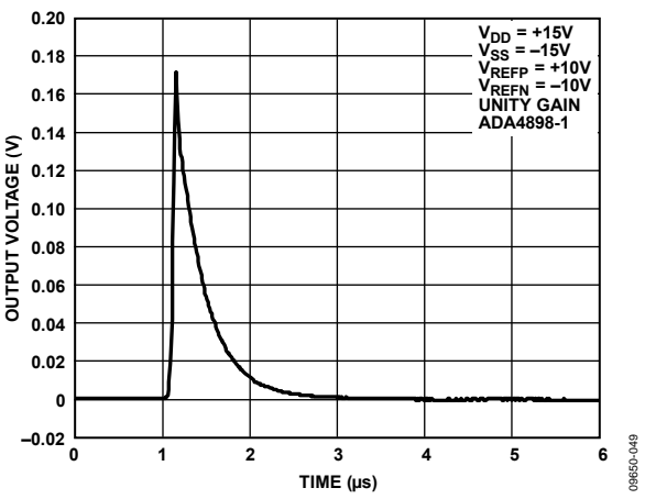
Figure 49. Glitch Impulse on Removal of Output Clamp
