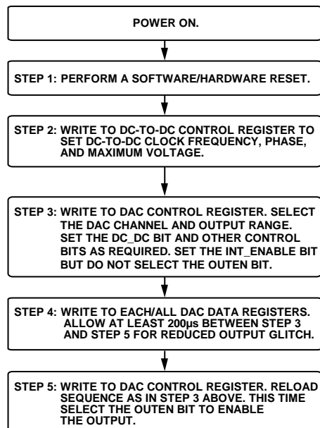
Figure 74. Programming Sequence for Enabling the Output Correctly
