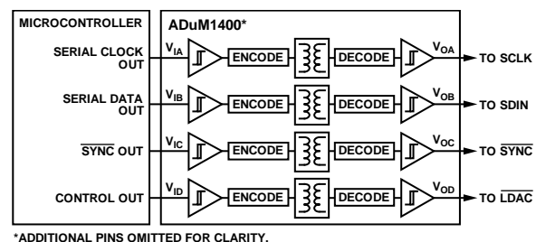
Figure 86. Isolated Interface
