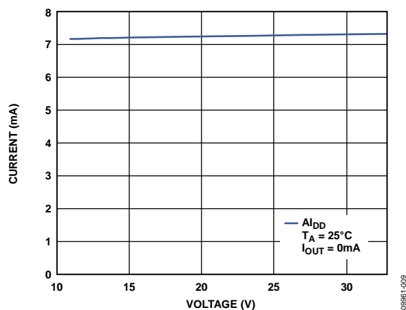
Figure 66. Supply Current ( A_{DD} ) vs. Supply Voltage ( AV_{DD} )
