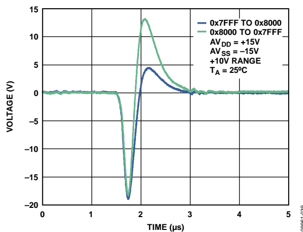
Figure 25. Digital-to-Analog Glitch
