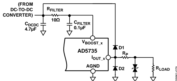
Figure 83. Output Transient Voltage Protection
