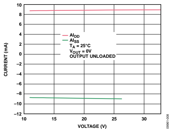
Figure 65. Supply Current ( A_{DD}/A_{SS} ) vs. Supply Voltage ( AV_{DD}/AV_{SS} )
