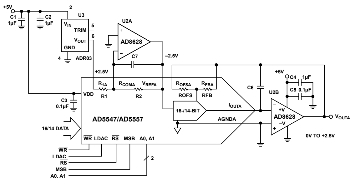
Figure 22. Unipolar 2-Quadrant Multiplying Mode, V_{OUT} = 0 to +V_{REF}
