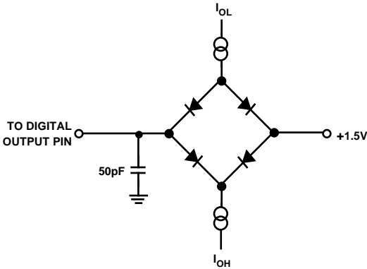
Figure 21. Equivalent Device Loading for AC Measurements (Includes ALI Fixtures)
