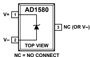
Figure 1. SOT-23
