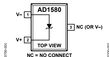
Figure 2. SC70
