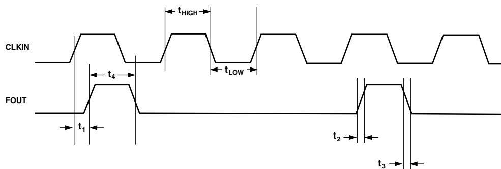
Figure 1. Timing Diagram
