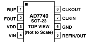
8-Lead SOT-23
