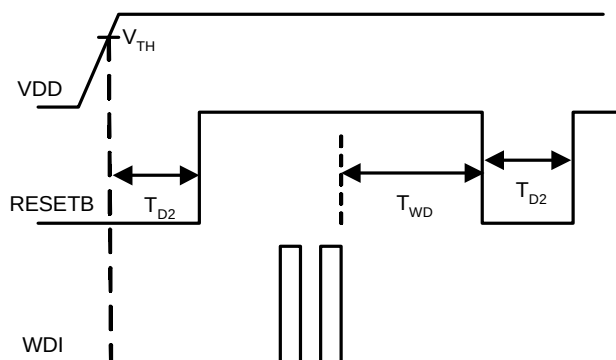
Watchdog Timing Diagram
