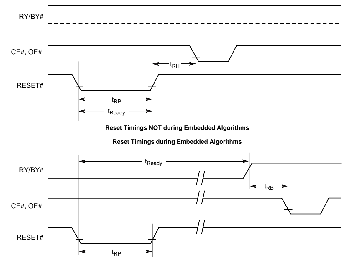
Figure 10. RESET# Timings
