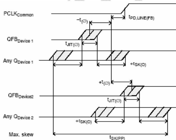
Figure 4. ASM5I9658 max device-to-device skew
