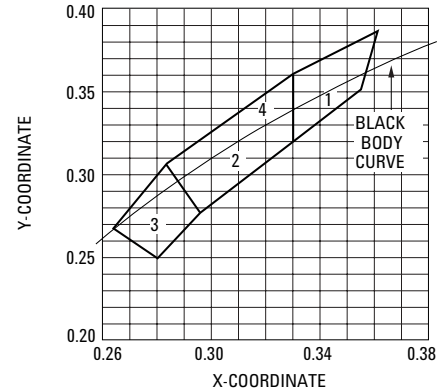
Color Bin Limits with Respect to CIE 1931 Chromaticity Diagram
