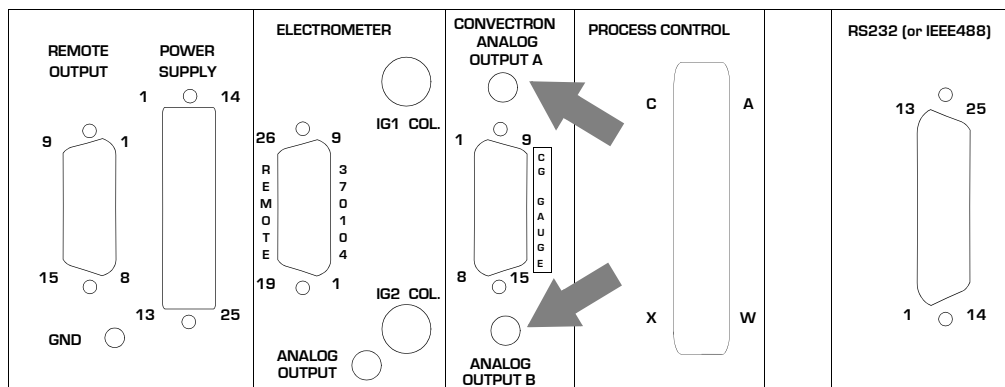
Figure 3-6 Convector Gauge Analog Output Connector Locations on the Rear Panel of the Controller
