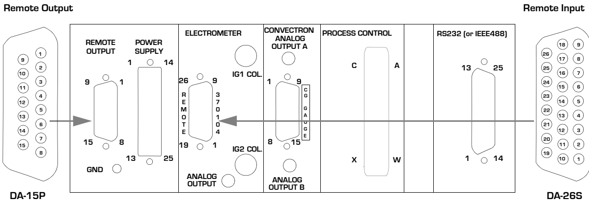
Figure 3-10 Control Unit Rear View Showing Locations of Remote Input and Output Connectors
