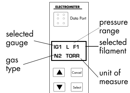
Figure 4-2 Electrometer Module with IG1 Status Menu on the Display
