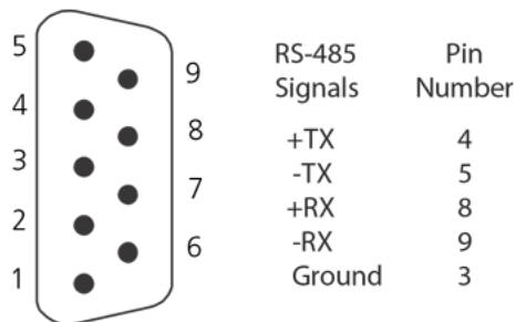
Figure 3-14 RS-485 Connector
