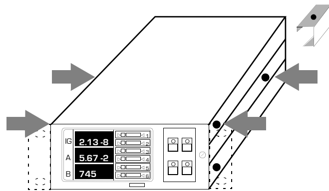
Figure 2-19 Location of Screws for Replacing Top Cover
