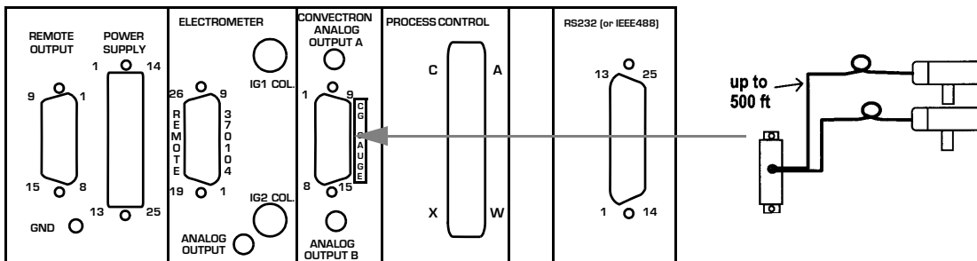
Figure 3-17 Control Unit Rear Panel Showing the Cable Connection to the Convector Gauges
