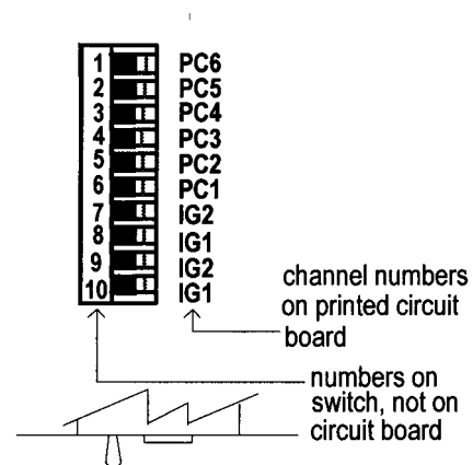
Figure 2-9 Partial Top View of Process Control Module
