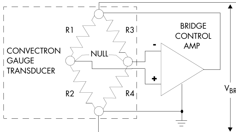
Figure 6-2 Simplified Schematic of Convectron Gauge
