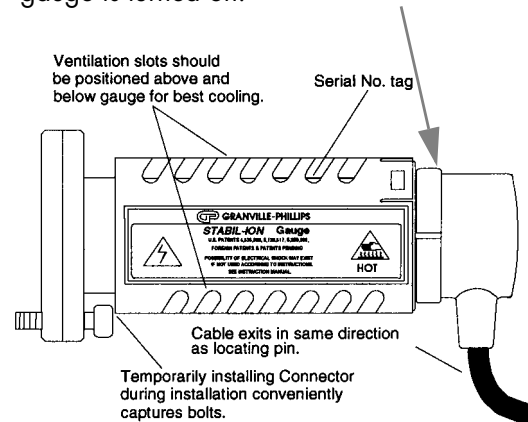
Figure 3-2 Stabil-Ion Gauge with Connector and Guard
