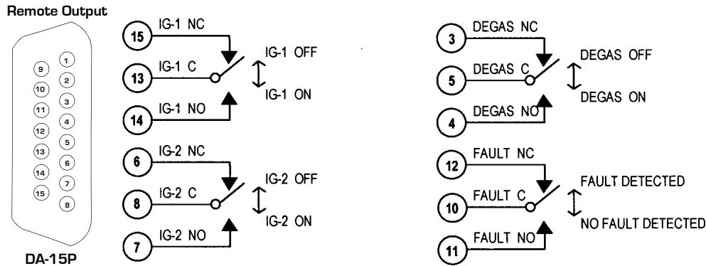
Figure 3-12 Remote Output Connector (Use DA-15S Mating Connectors, Supplied)
