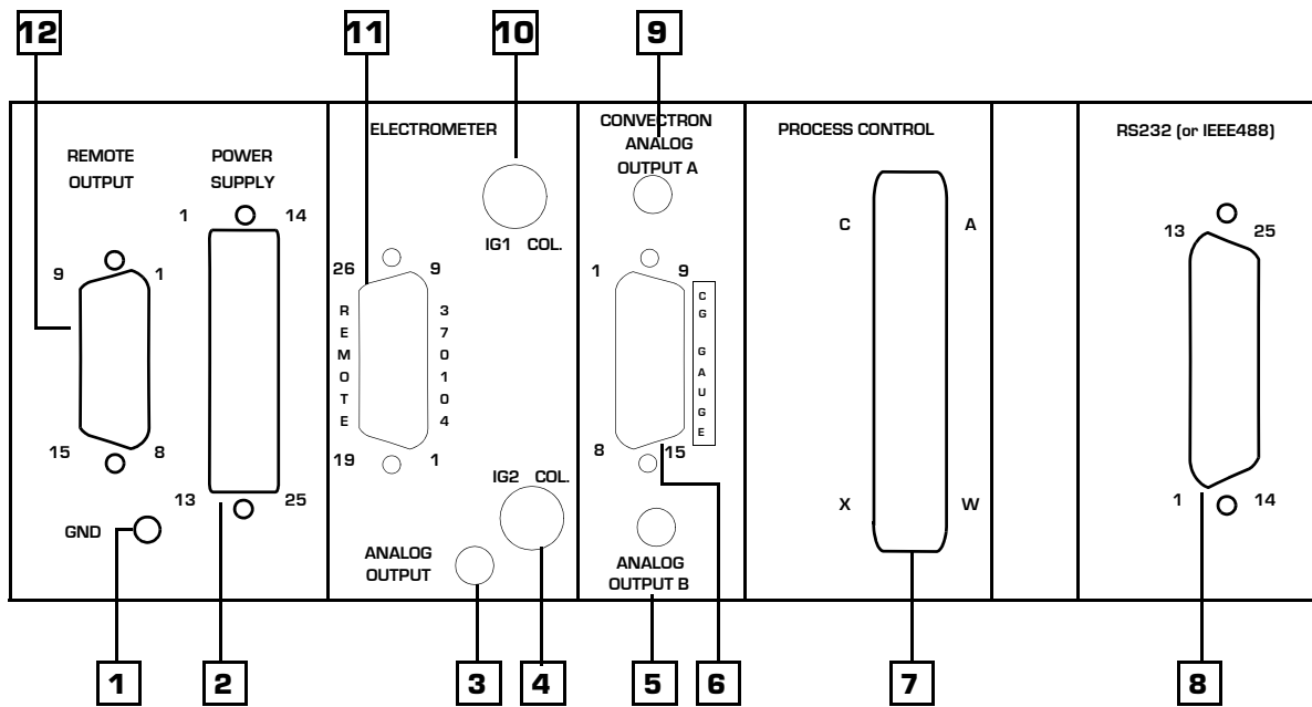
Figure 1-6 Stabil-Ion Vacuum Gauge Control Unit Rear Panel
