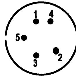
Figure 7-3 Convectron Gauge Base
