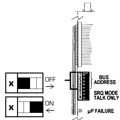
Figure 2-16 Top View of IEEE 488 Module
