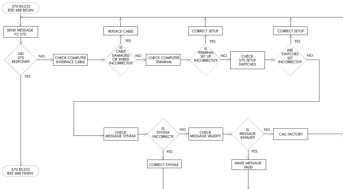
Figure 7-11 RS-232/IEEE 488 Interface
