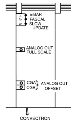
Figure 4-18 Top View of Convector Gauge Module Showing Analog Output Offset Adjustment
