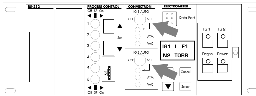
Figure 4-15 Control Unit Front Panel (with Door Open) Showing Ionization Gauge Auto Turn-On/Off Switches
