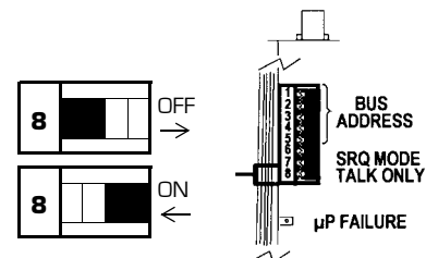
Figure 2-17 Top View of IEEE 488 Module
