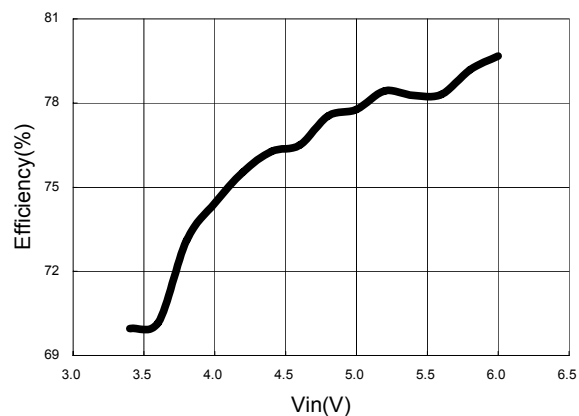
Efficiency vs Vin (9WLEDs)
