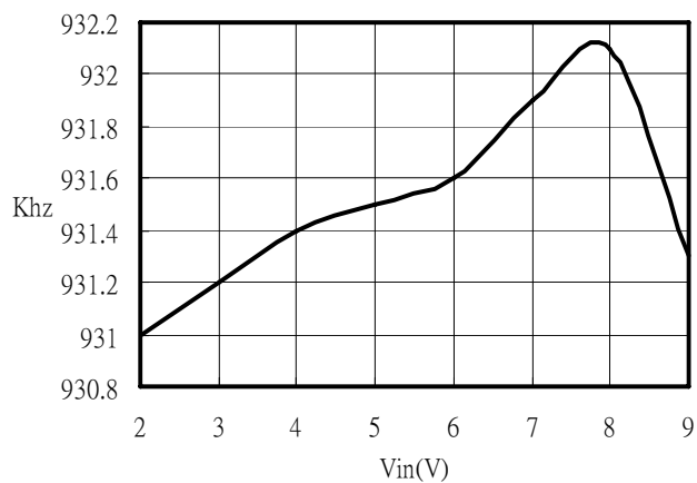
Switching Frequency
