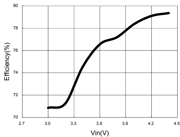
Efficiency vs Vin (7WLEDs)
