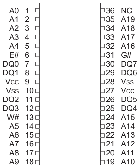
Pin Configuration
