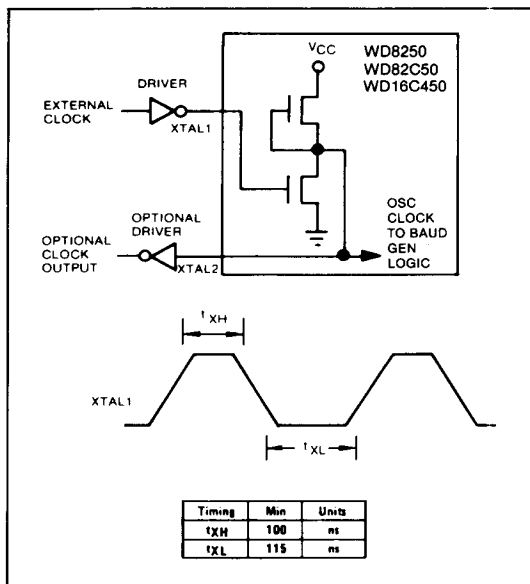
FIGURE 5. EXTERNAL CLOCK INPUT (3.1 MHz MAX.)
