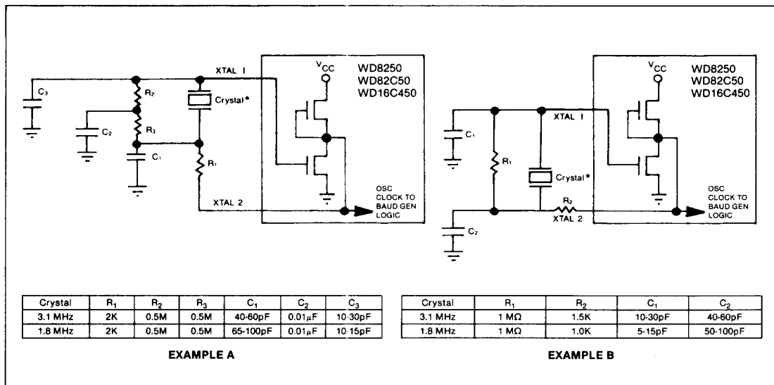
FIGURE 6. TYPICAL CRYSTAL OSCILLATOR NETWORKS
