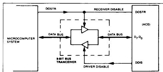
FIGURE 3. TYPICAL INTERFACE FOR A HIGH-CAPACITY DATA BUS
