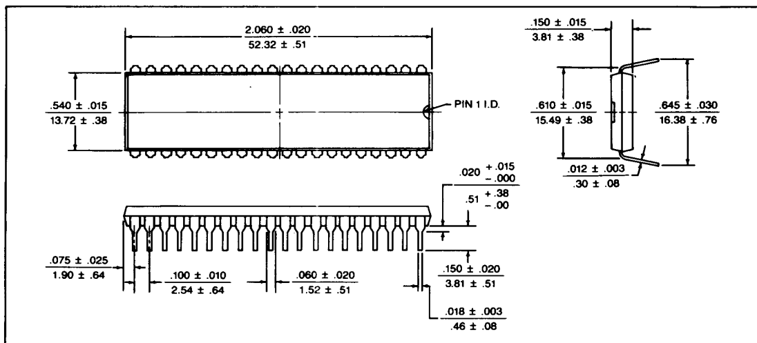
40 LEAD PLASTIC "PL"
