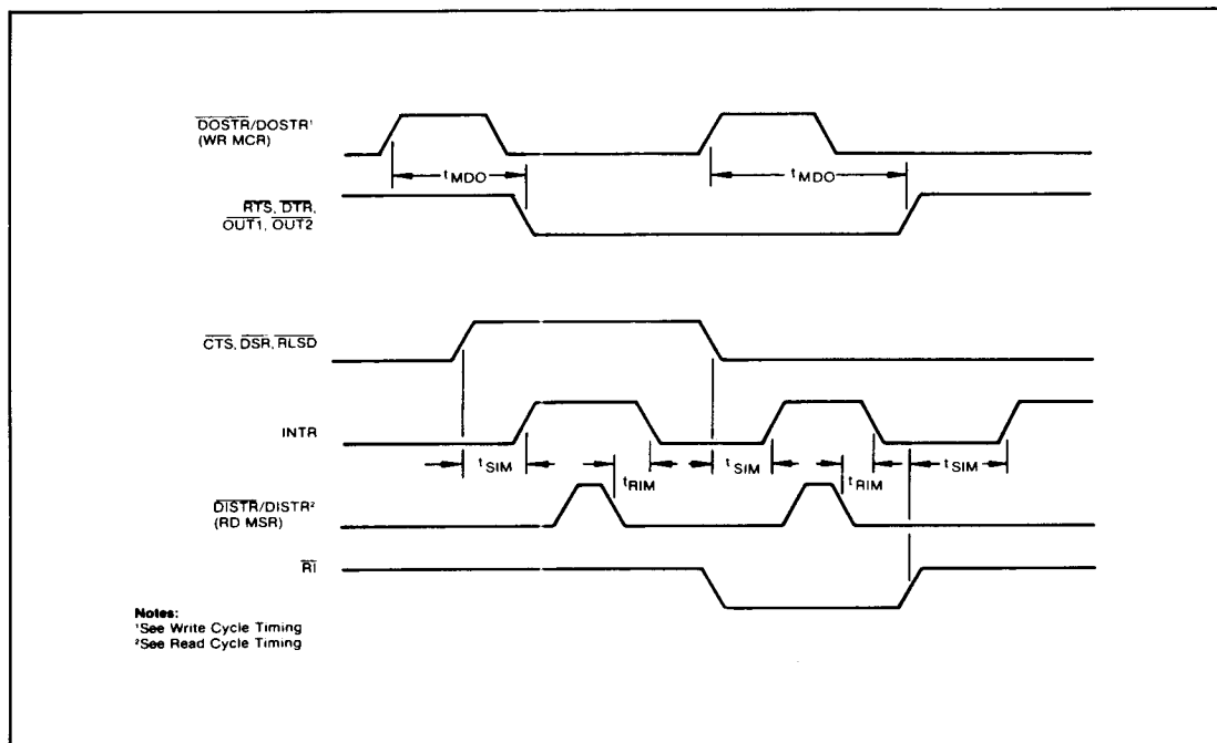
FIGURE 10. MODEM CONTROL TIMING
