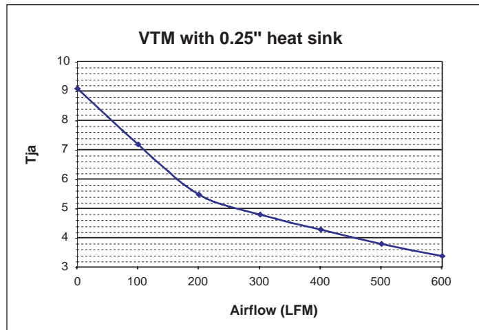
Figure 18 —Junction-to-ambient thermal resistance of VTM with 0.25 inch Heat Sink.
