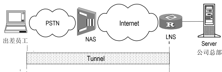
图2-7 Client-Initialized VPN 组网图
