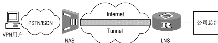
图2-6 NAS-Initialized VPN 组网图
