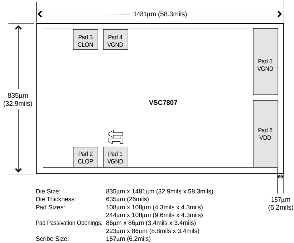
Figure 2: Pad Assignments
