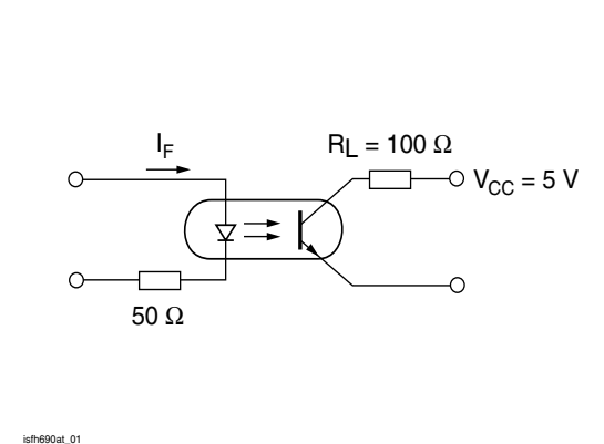
Figure 2. Switching Operation (without Saturation)
