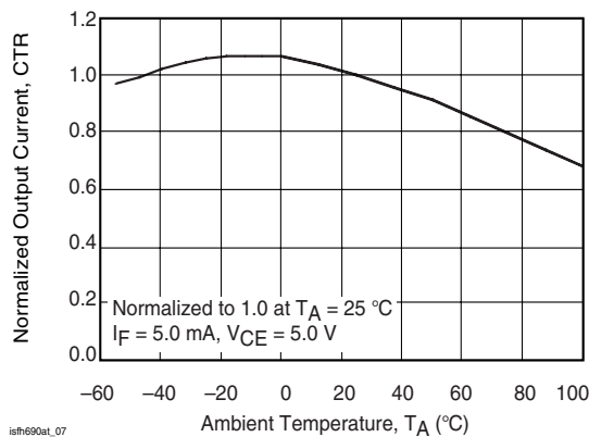
Figure 8. Normalized Output Current vs. Ambient Temperature
