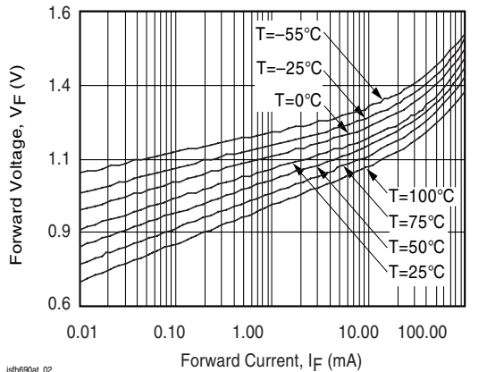
Figure 3. Diode Forward Voltage vs. Forward Current
