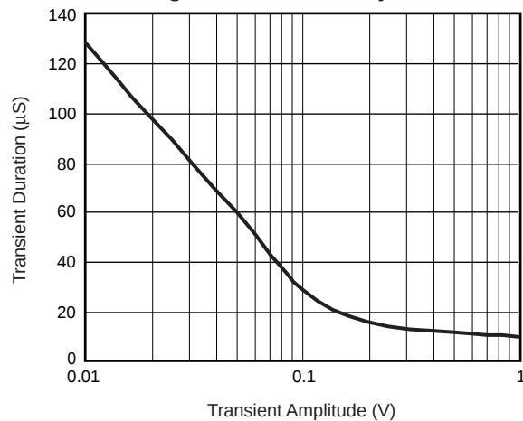
Fig. 3 – Transient Rejection
