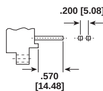
Type "K" Wire Wrap™, Standard .025 [.635] Square Terminals
