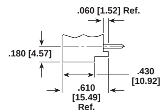
Type "W" No Mounting Flange
