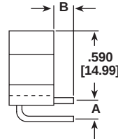
Type "1R", "2R", "3R" and "4R" Right Angle .025 [.635] Square Terminals
