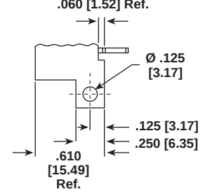
Type "W" No Mounting Flange
