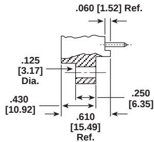
Type "Y" Threaded Insert Raised Mounting Flange
