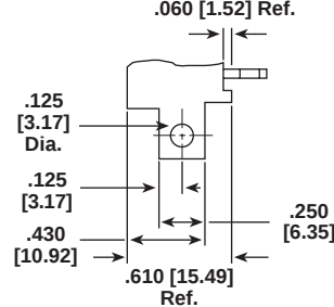
Type "YF" Threaded Insert Flush Mounting Flange
