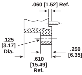
Type "YF" Threaded Insert Flush Mounting Flange
