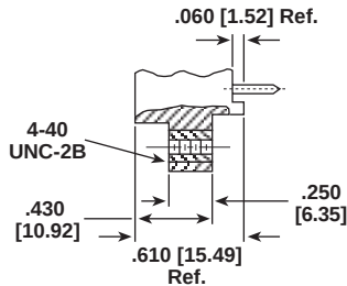
Type "Y" Threaded Insert Raised Mounting Flange
