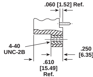
Type "YF" Threaded Insert Flush Mounting Flange
