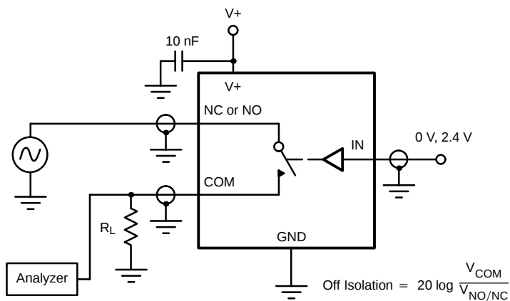
FIGURE 3. Off-Isolation
