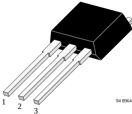
BUD7312 1 Base 2 Collector 3 Emitter
