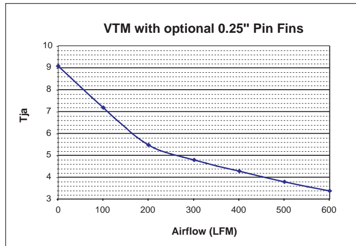
Figure 18 —Junction-to-ambient thermal resistance of VTM with 0.25 inch Pin Fins. (Pin Fins are available as a separate item.)
